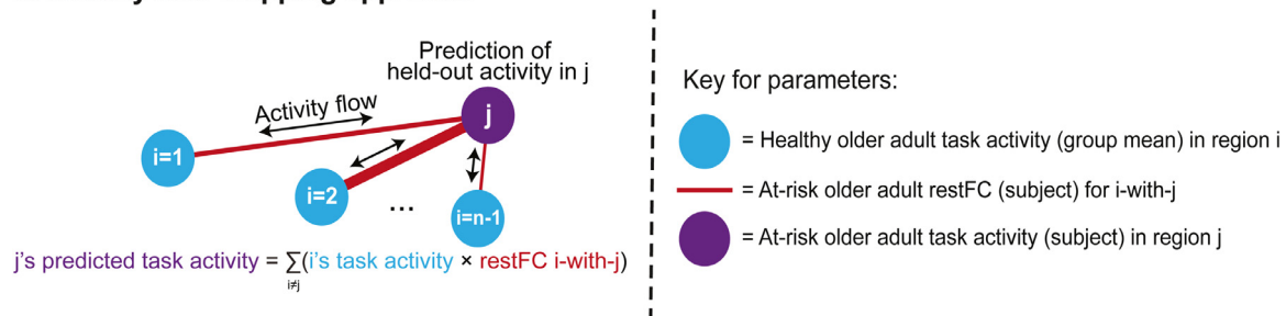
Fig. 1. Theoretical and methodological principles underlying application of activity flow mapping in an integrated connectivity-activity account of at-risk Alzheimer's disease (AD). a) Abstract theoretical underpinnings of activity flow mapping – which is based on the core mechanism underlying neural network simulations – in a clinical context. A 'healthy' aged task activation pattern is transformed into an 'unhealthy' aged activation (i.e. one associated with being at-risk for developing AD) by an altered pattern of resting-state functional connectivity (restFC) in at-risk subjects disrupting the ability for task activations to flow between brain regions. b) Methodological formalization of the activity flow mapping approach. Task activation in a held-out brain region ( j ) in a held-out at-risk AD subject is predicted from the dot product between the healthy activation state of the rest of the brain (regions i , estimated as the mean activation in the healthy group) and the restFC between i and j (estimated from the to-be-predicted at-risk subject). See Methods for further details.
